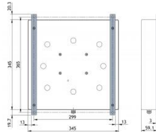
MOUNTING DETAILS (PATCH-WAMO)
