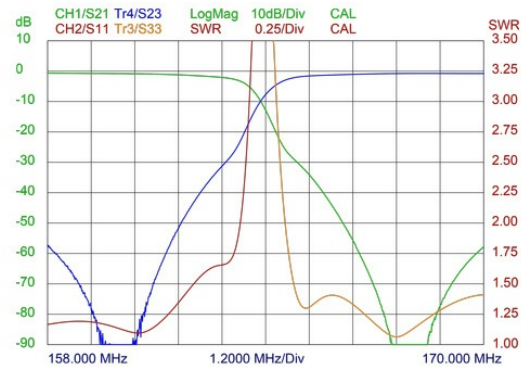
TYPICAL RESPONSE CURVES @ 8 MHZ DUPLEX SPACING
