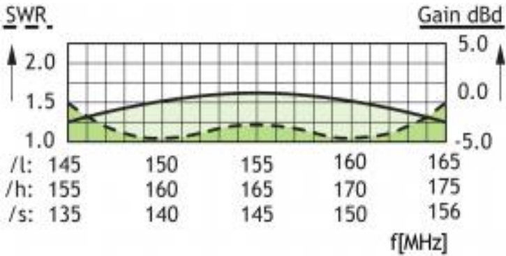
TYPICAL GAIN AND SWR CURVES
